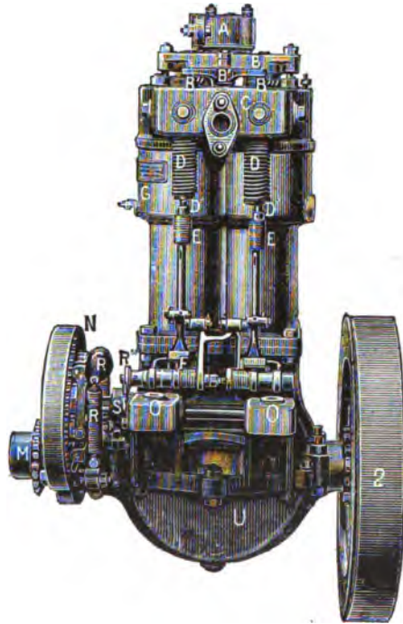
FIG. 375.—The Phenix-Daimler Double-vertical Cylinder Carriage Motor, as used by Panhard-Levassor. A is the port for admitting fuel gas under piston suction; B, the inlet valve; B', the exhaust valve; C, the ignition apparatus; D, spring on the exhaust valve; D', exhaust valve rod; E, pushrod actuated by the cam; F, governor attachment; N, wheel on the cam shaft, carrying the governor; R, the centrifugal weights of the governor; R', the governor springs; R'', sliding cam shaft; S, the cam actuating the exhaust valves; U, the engine flywheel carrying the female cone of the main clutch.
